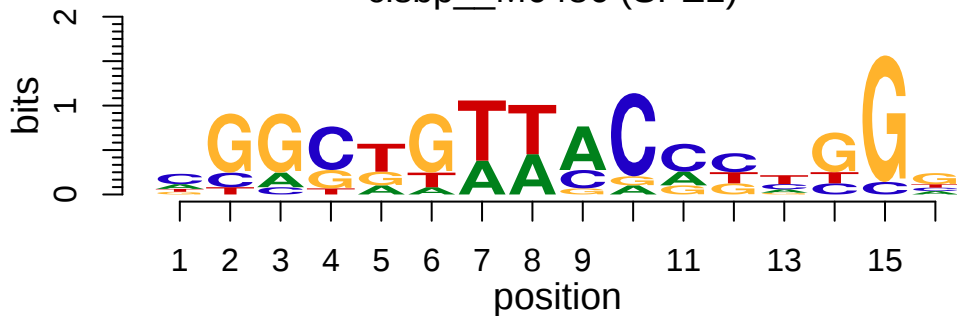
cisbp__M6486 (SPZ1)
