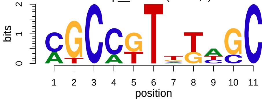
cisbp__M4261 (ARG5,6)
