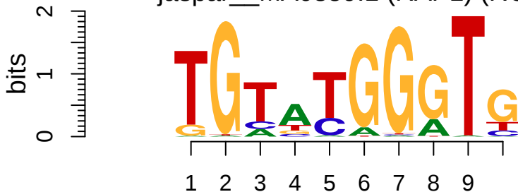
jaspar__MA0359.1 (RAP1) (RC)
