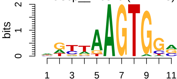
cisbp__M6379 (NKX2-3)
