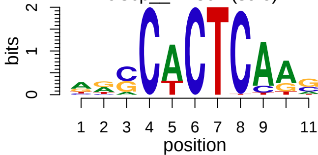
cisbp_M2302 (scro)
