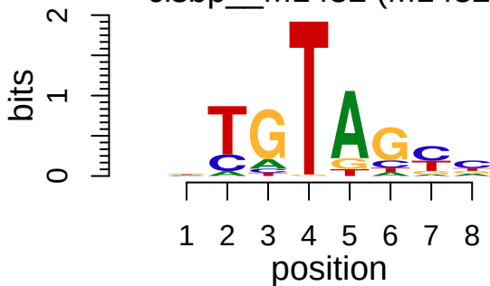
cisbp__M1482 (M1482)
