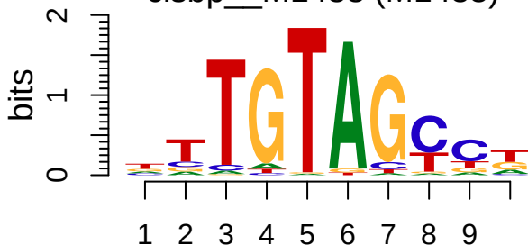
cisbp__M1488 (M1488)
