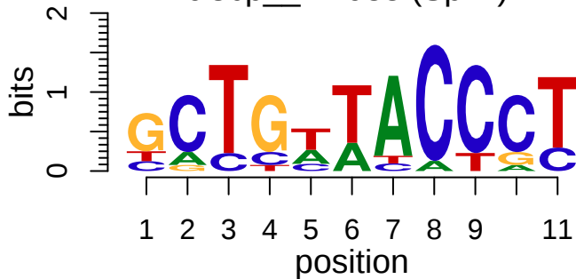
cisbp__M1933 (Spz1)
