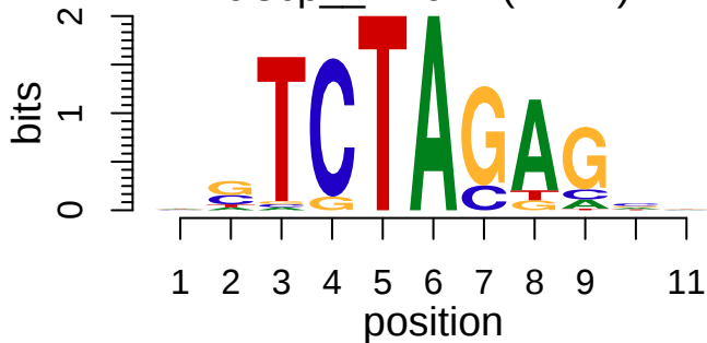
cisbp_M1614 (ABF2)
