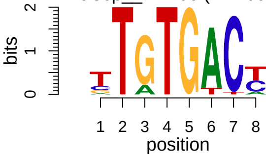
cisbp_M1466 (M1466)
