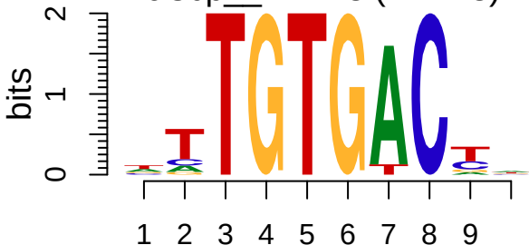
cisbp_M1478 (M1478)
