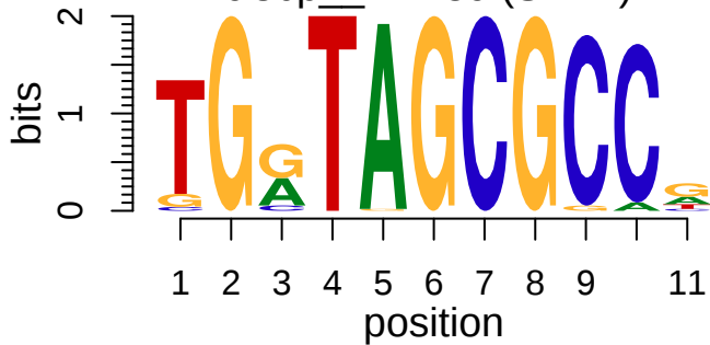
cisbp_M2189 (SNT2)
