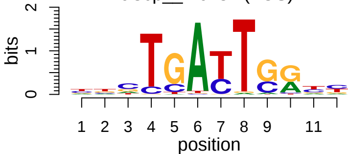
cisbp__M6231 (FOS)
