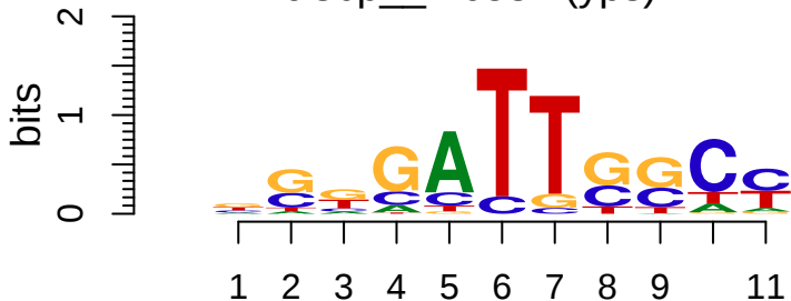
cisbp__M6537 (yps)
