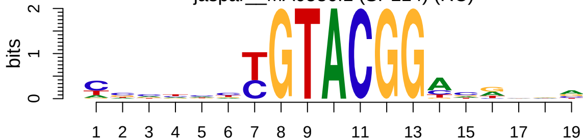
jaspar__MA0586.1 (SPL14) (RC)
