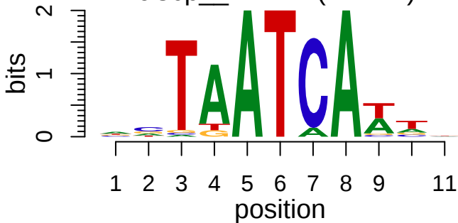
cisbp_M1212 (M1212)
