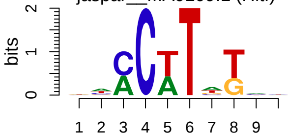
jaspar__MA0109.1 (Hltf)
