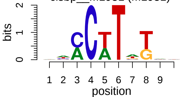
cisbp__M1931 (M1931)
