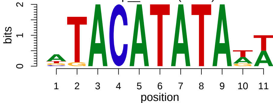
cisbp_M4232 (PDC2)
