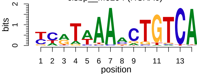
cisbp__M6294 (HOXA6)
