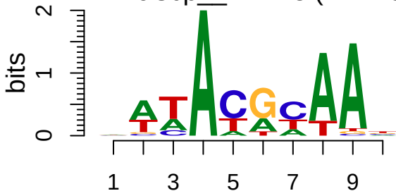
cisbp_M1415 (M1415)
