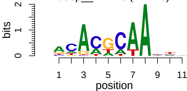
cisbp_M1413 (M1413)
