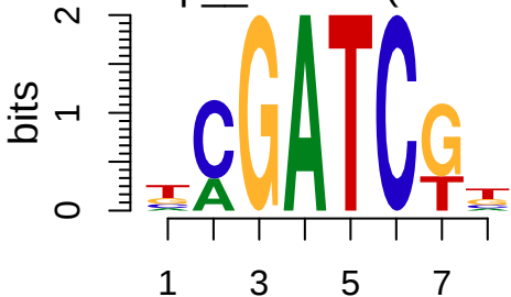
cisbp_M0779 (M0779)
